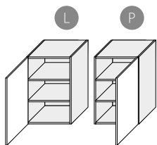
W2/50 500/720/325
