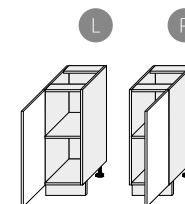
D1D/30 300/820/500
