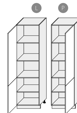
D14/DP/60/207 600/2070/565
