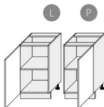
D1D/45 450/820/500
