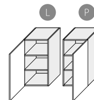
W2/40 400/720/325
