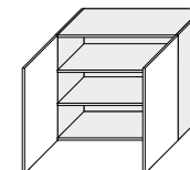
W3/90 900/720/325
