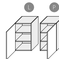
W2/45 450/720/325
