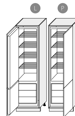
D14/DL/60/207 600/2070/565
